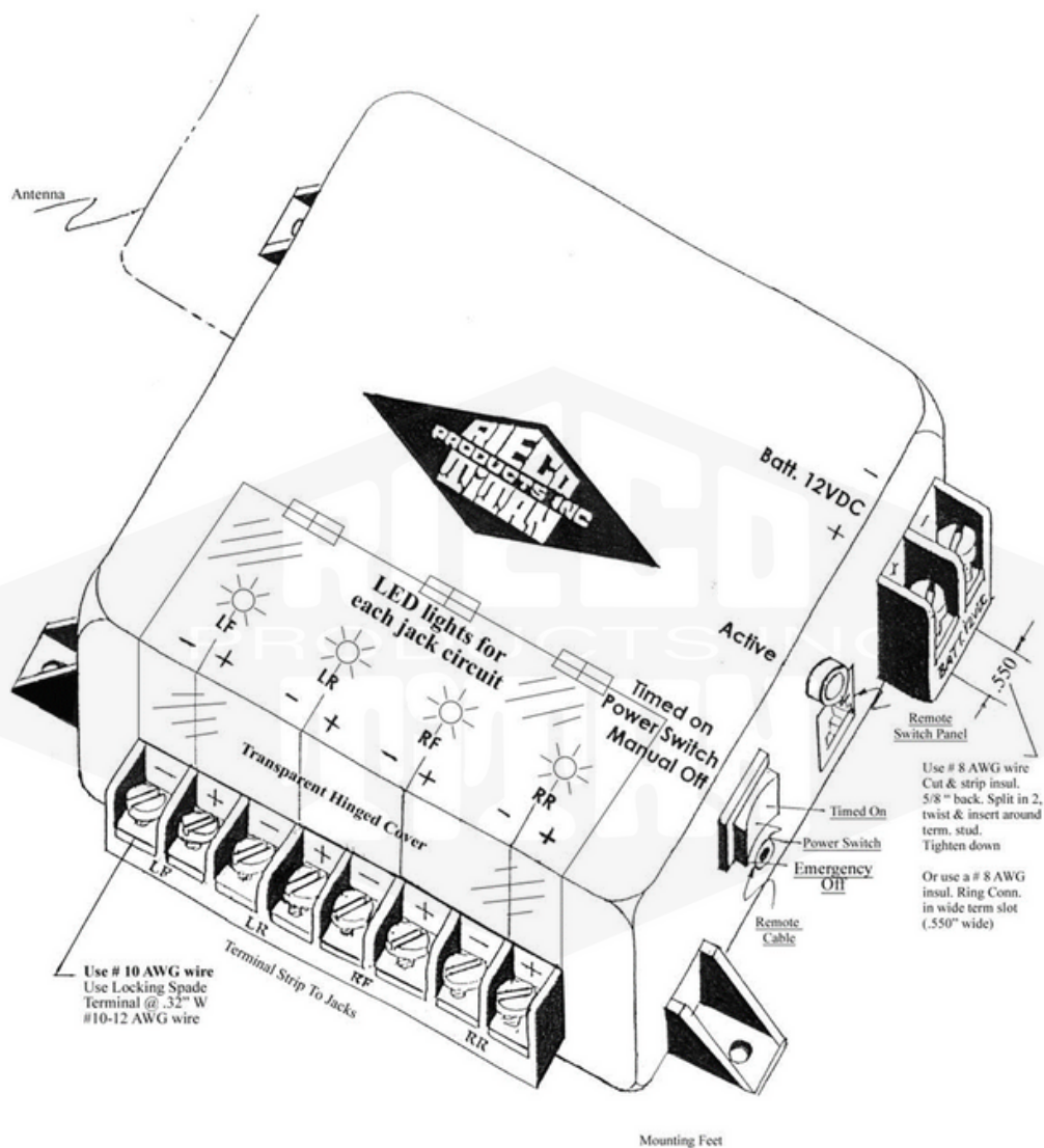
WIRED-WIRELESS RECEIVER CONTROL BOX
